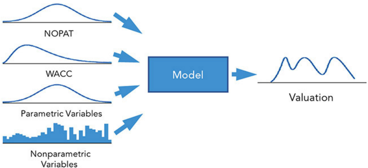
(B) Distributions as inputs producing a distribution as an output
