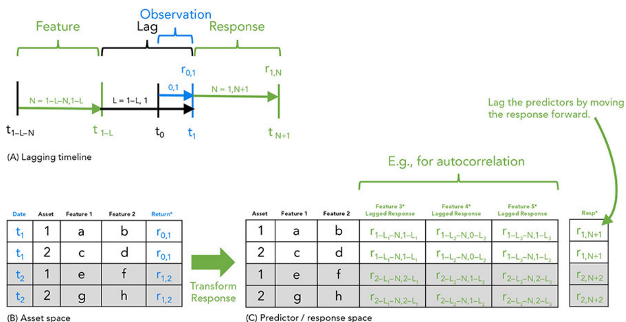
FIGURE 9-1 Transforming the response to remove time stamps and avoid look-ahead bias
