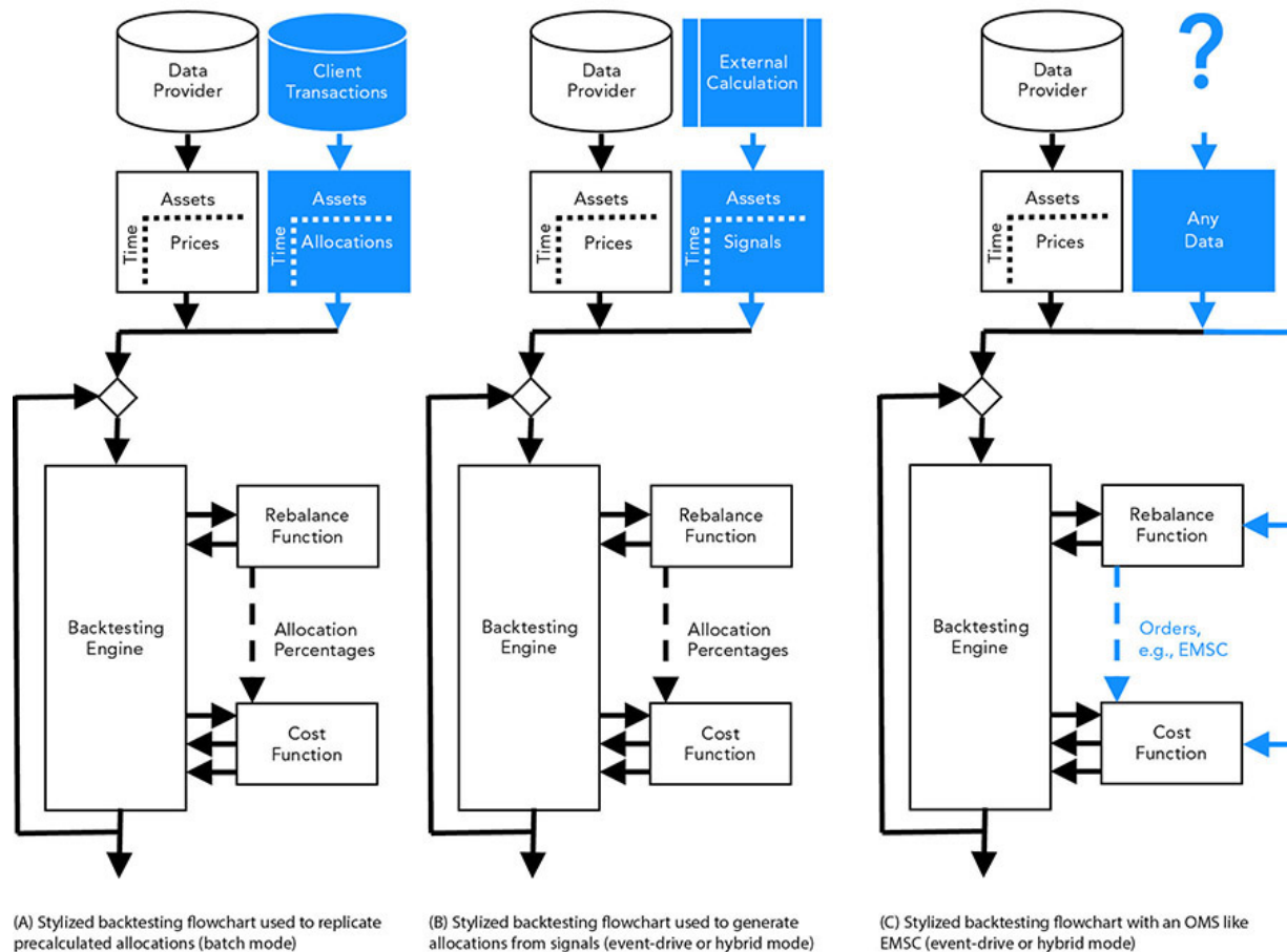
FIGURE 14-1 Operating modes of a backtester
