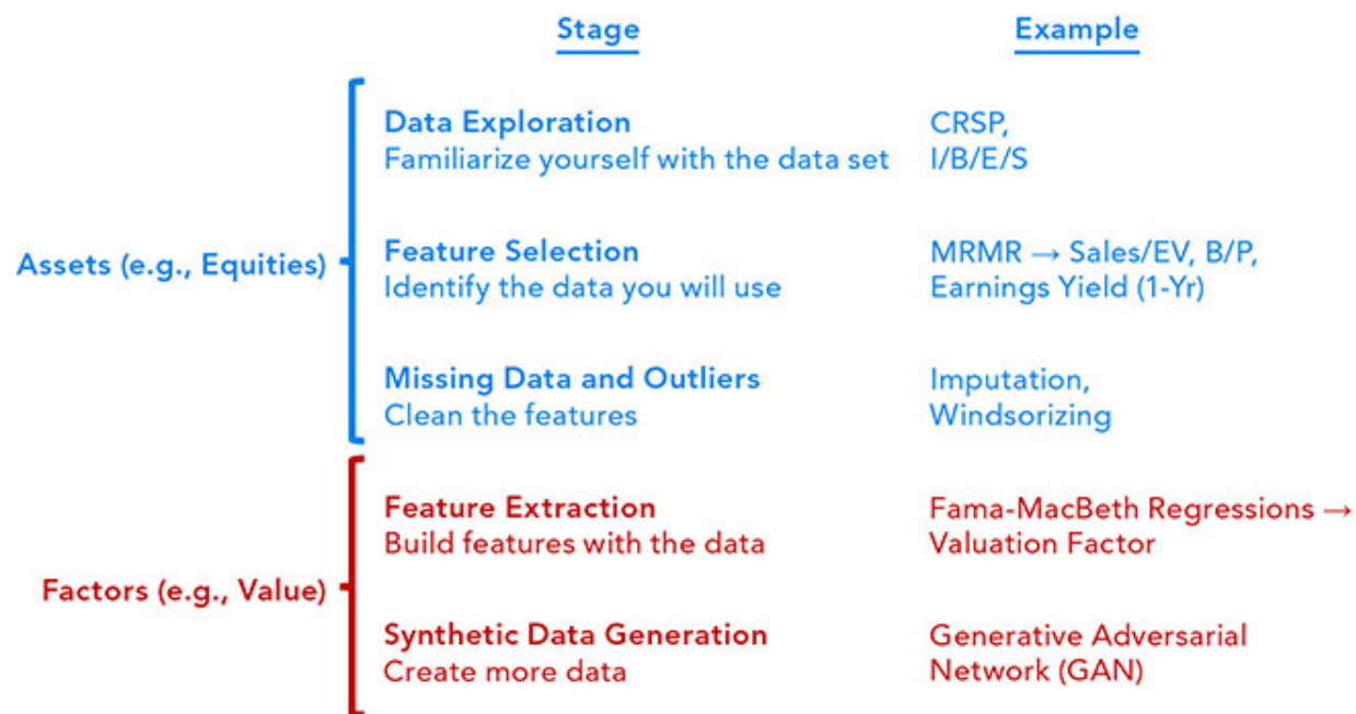
FIGURE 6-1 The feature engineering process
