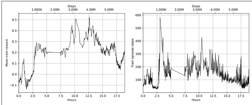
Figure 17.2: The reward (left) and steps (right) for training episodes
