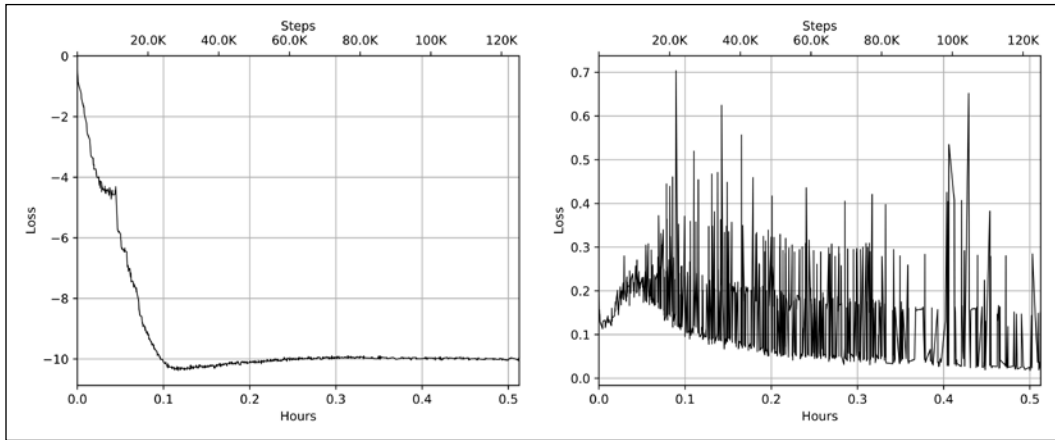
Figure 18.10: The loss of the actor (left) and critic (right)
